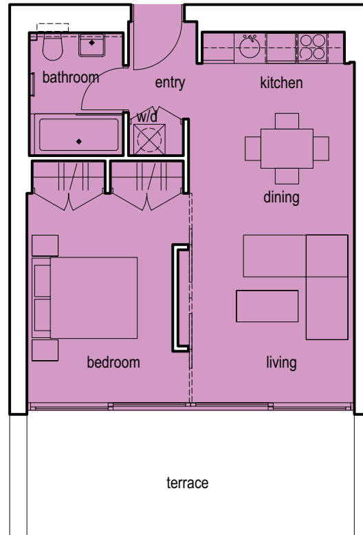
1 Bedroom - Type 1 Internal Area 51 m 2 Terrace Area 16 m 2
